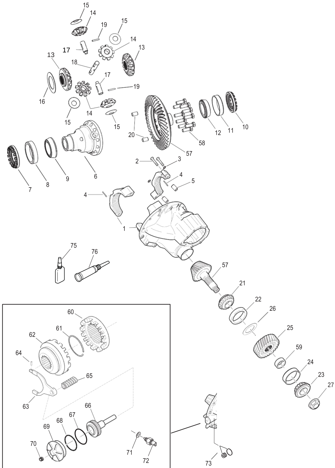
WHEEL DIFFERENTIAL LOCK SHIFT PARTS
