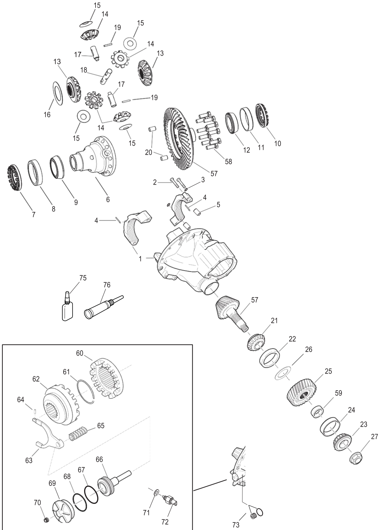
WHEEL DIFFERENTIAL LOCK SHIFT PARTS
